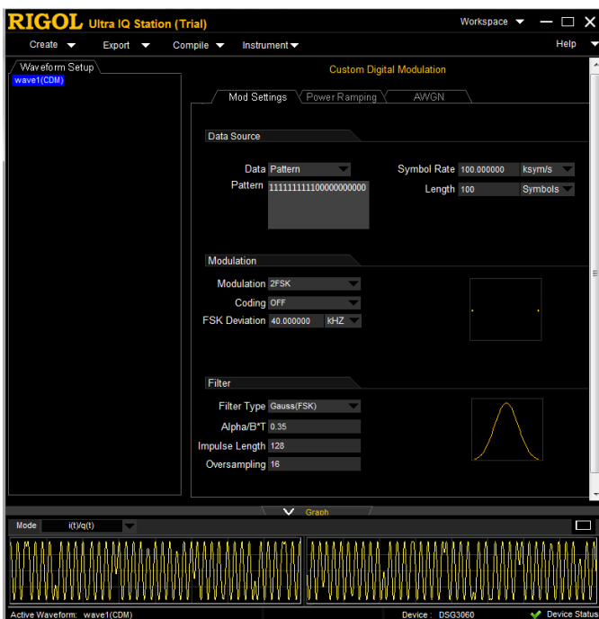
Figure 7: 2FSK Signal generation with ULTRA IQ STATION
