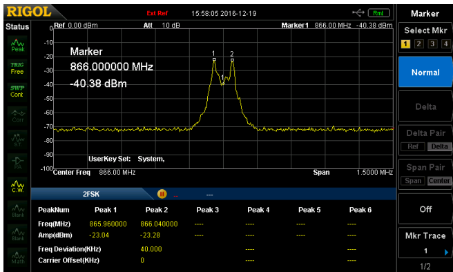
Figure 1: 2FSK measurement with DSA815 and SSC option
