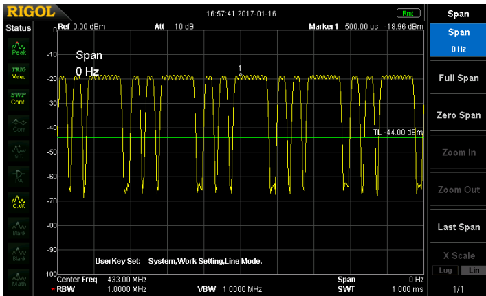
Figure 18: Zero Span analysis of ASK Signal
