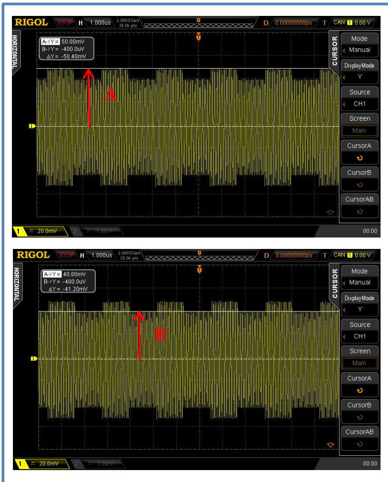
Figure 15: ASK modulation of 10%
