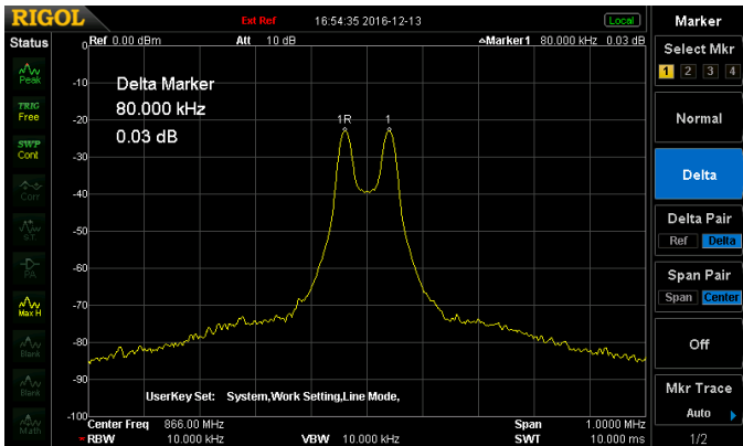
Figure 1: 2FSK Signal with FSK deviation of 40 kHz, fcarrier = 866 MHz, tested with DSA832E
