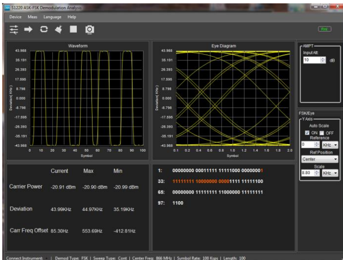
Figure 8: Software S1220 for ASK / FSK demodulation
