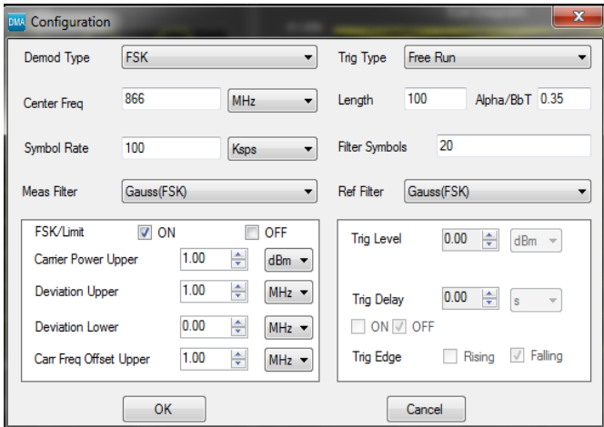
Figure 9: FSK configuration in S1220
