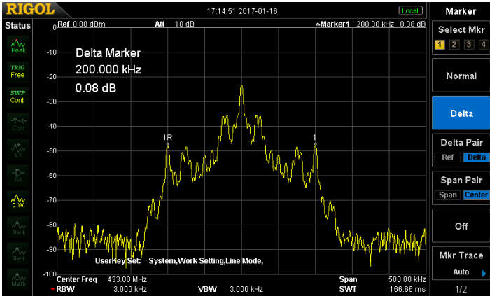
Figure 17: Spectrum of ASK
